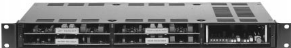
SP23-30 (1/3 Octave Equalisers) card positions
